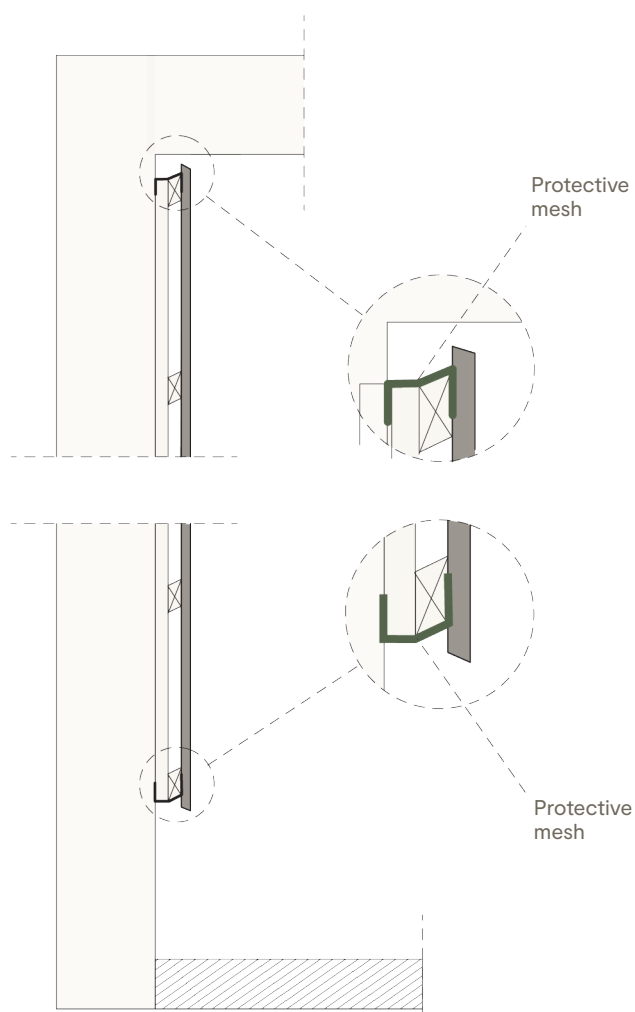
Fig. 2: Protective mesh for vertical cladding on a double-layer frame
