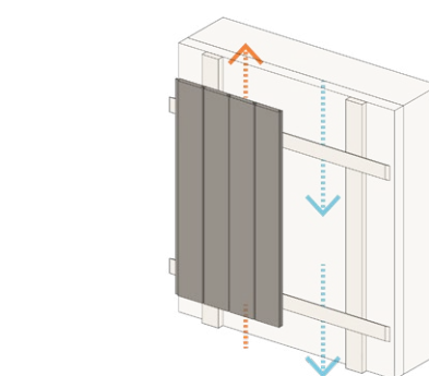
Fig. 2: Double-layer frame when cladding boards are installed vertically
