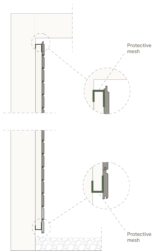
Fig. 3: Protective mesh for horizontal cladding on a single-layer frame
