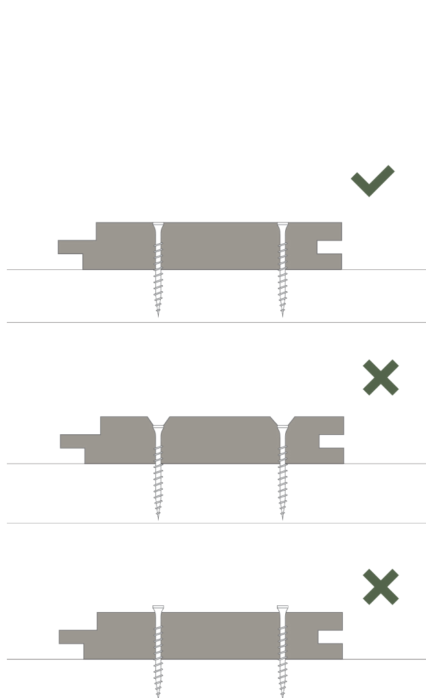
Fig. 1: The head of the wood screw or nail must be flush with the cladding board
