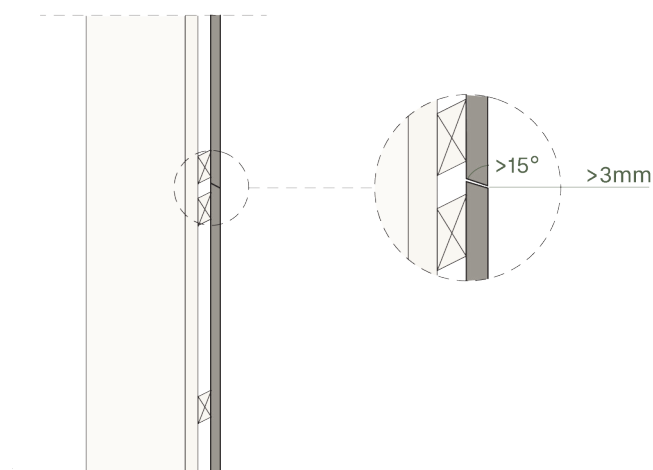
Fig. 2: Joint detail of cladding with a ventilation gap
