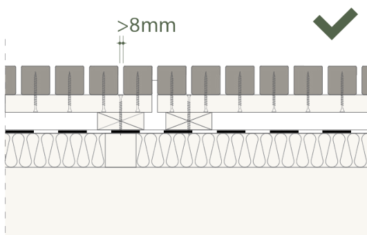
Fig. 2: Correct installation onto vertical battens
