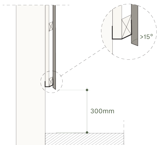
Fig. 3: Bottom edge detail of cladding and the recommended clearance from the ground
