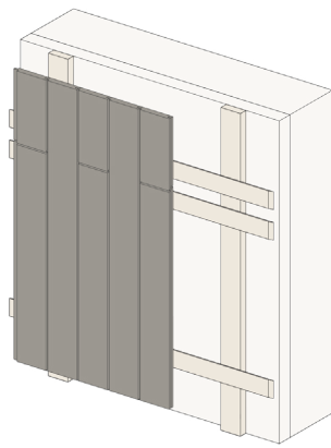
Fig. 1: Double horizontal batten at cladding board joints
