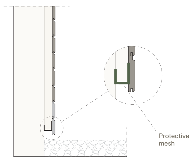
Fig. 3: Protective mesh for horizontal cladding on a single-layer frame
