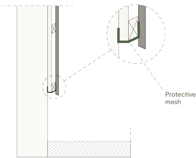
Fig. 2: Protective mesh for vertical cladding on a double-layer frame
