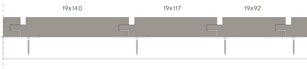
Fig. 2: Fastening of cladding boards using hidden fixings
