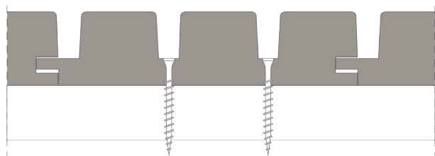
Fig. 1: Fastening GRÊTÈ cladding through the board
