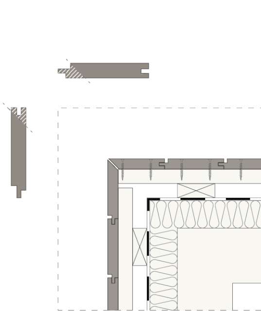
Fig. 1: External corner finishing by cutting the board edges at a 45° angle
