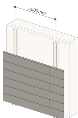
Fig. 1: Single-layer thermo subframe for horizontal cladding installation
