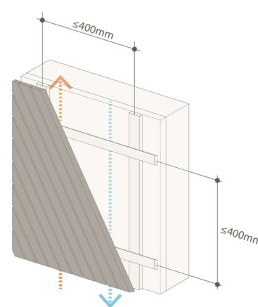
Fig. 4: Double-layer frame when cladding boards are installed at an angle greater than 45^\circ
