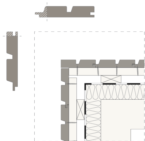
Fig. 3: External corner finishing by cutting off both the tongue and groove edges of the two connecting boards
